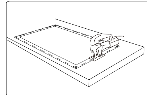
Cut along this dotted line to connect holes
