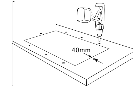
Drill eight holes on the back φ 10 with depth 15mm on the back
