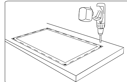
Drill four corner holes - 1/2" Diameter
