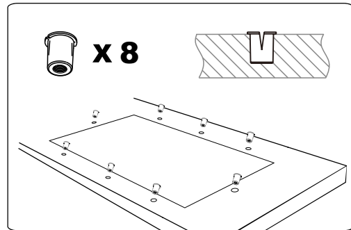
Anchor
