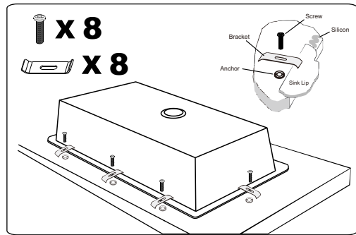
Locate
