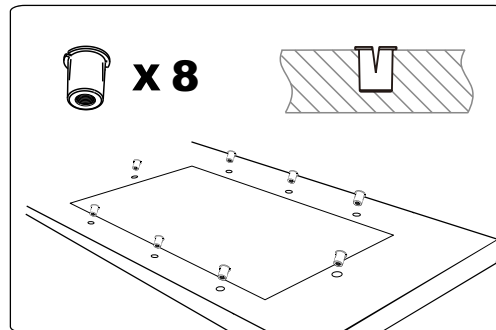
Anchor
