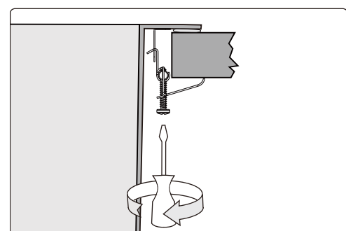
Tighten All
