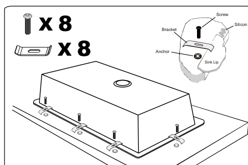
Locate
