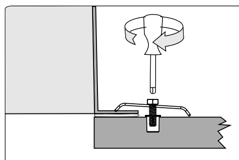
Tighten All
