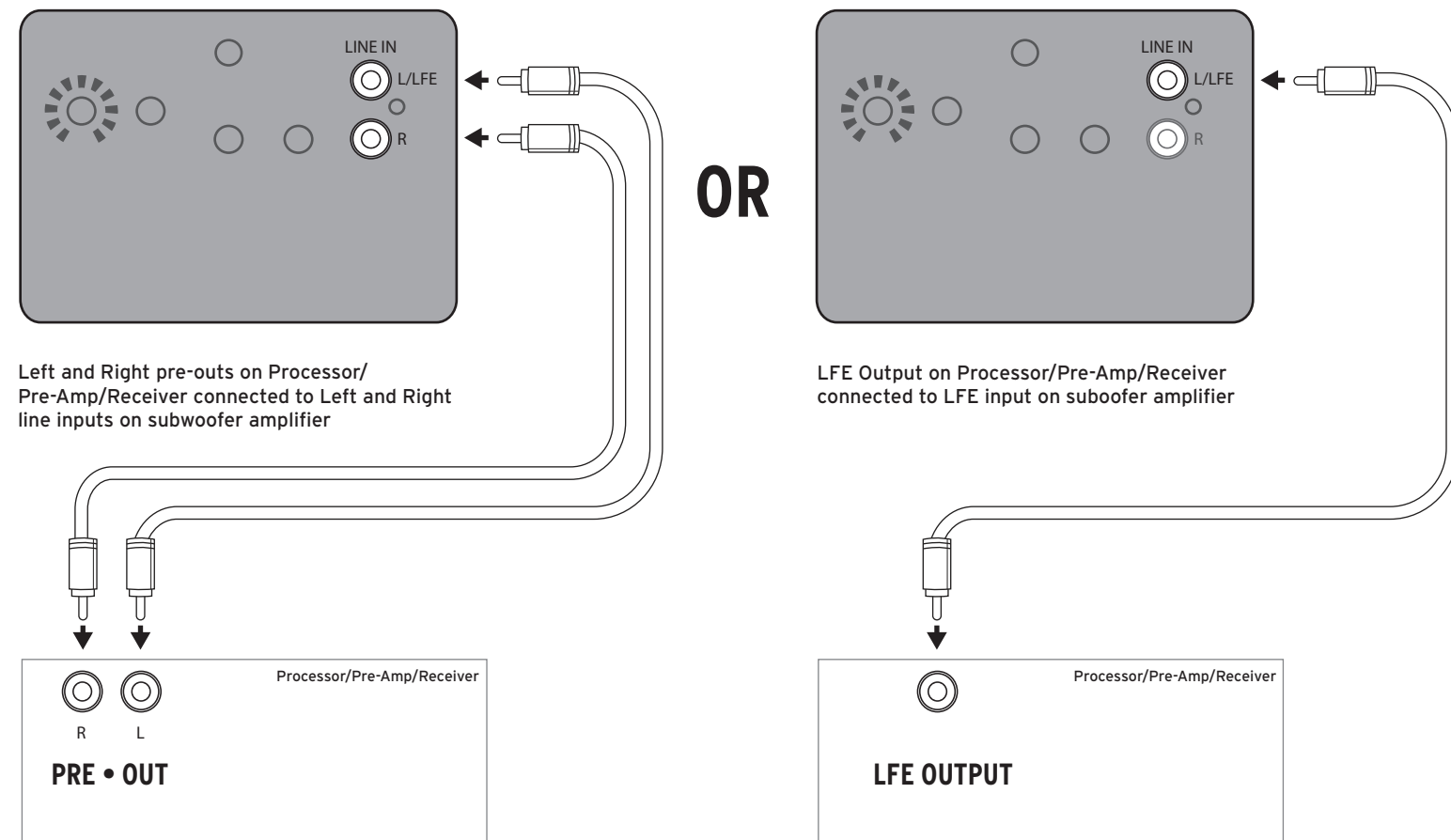
FIGURE 2 LINE LEVEL CONNECTIONS
