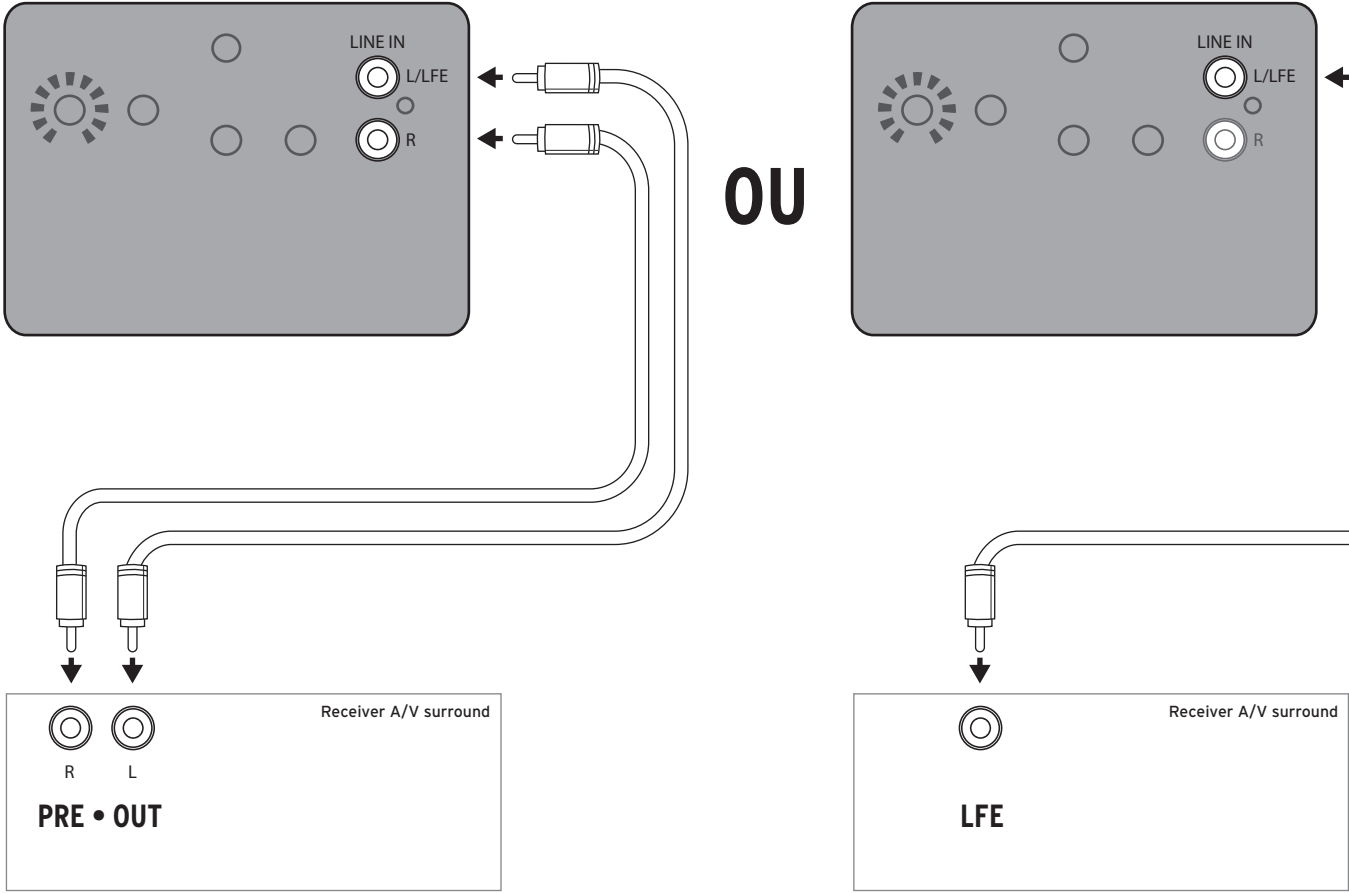
FIGURA 2 CONEXÃO DO SUBWOOFER R-100SW, R-120SW
